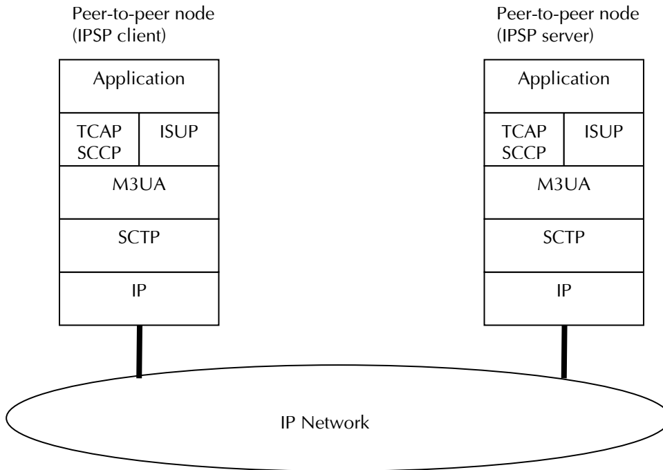
Figure 11 - M3UA peer-to-peer
